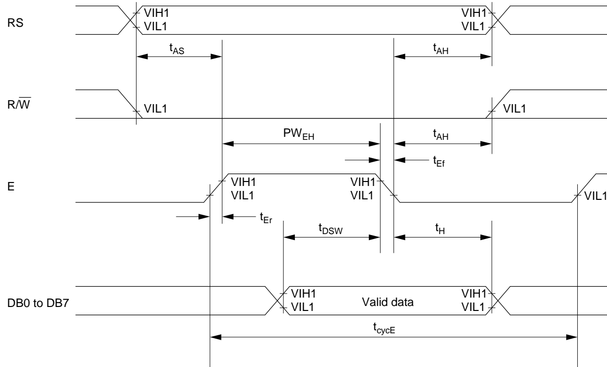
Figure 27 Write Operation
